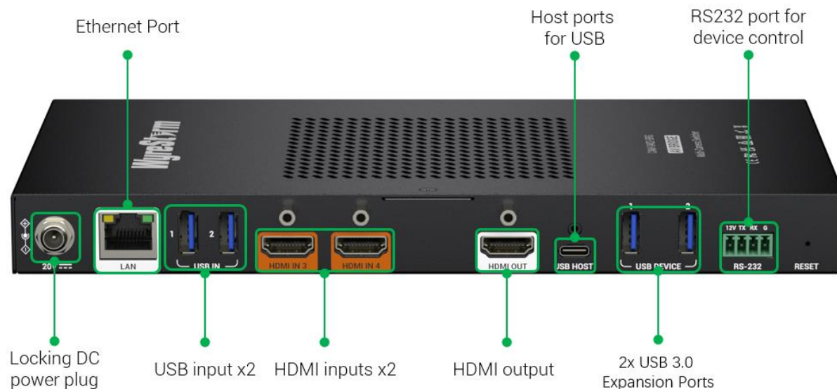
Rear Panel
